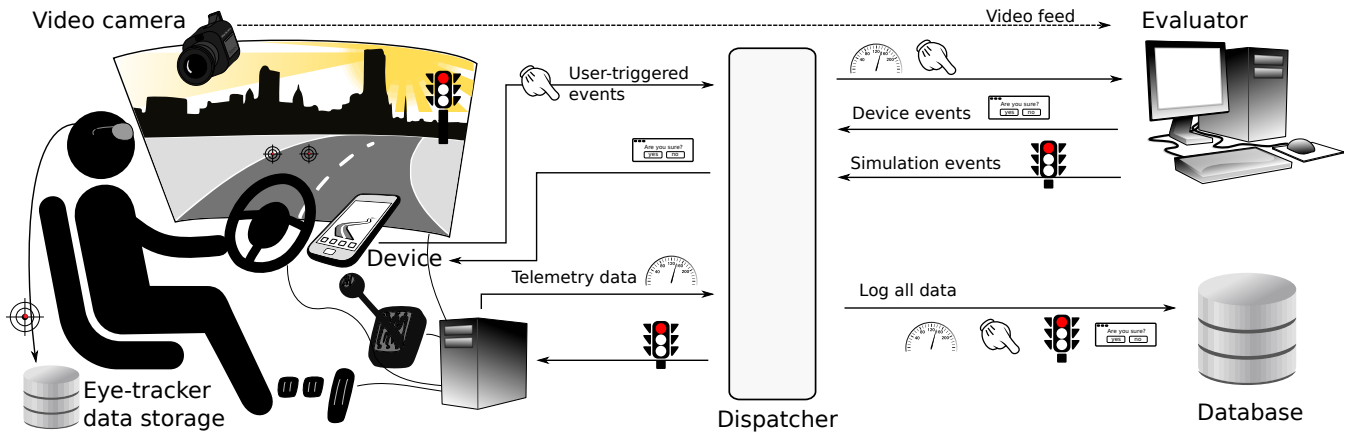
Figure 1: A scheme of the simulator usage in I-GEAR
